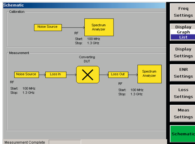
Test setup (schematics).
